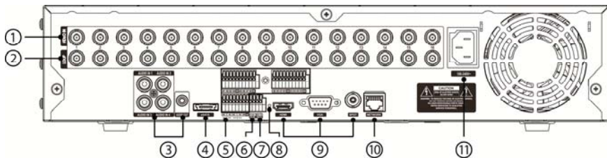
Figure 2: 16-Channel DVR rear panel.
