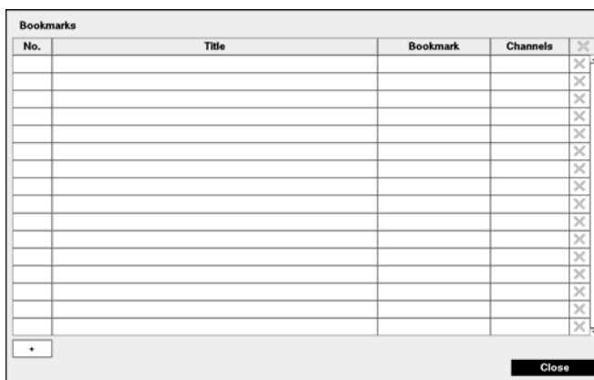
Figure 52: Bookmarks screen.
