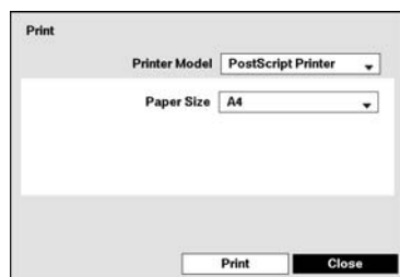
Figure 54: Print screen.
