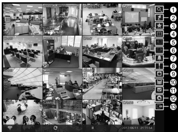
Figure 47: Search menu.
