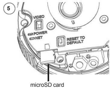
microSD card
