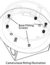
Camera base fitting illustration
