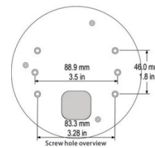
Camera base fitting illustration
