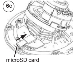
microSD card
